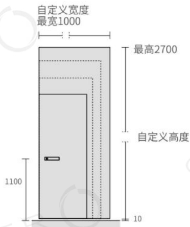
STM024尺寸范围
