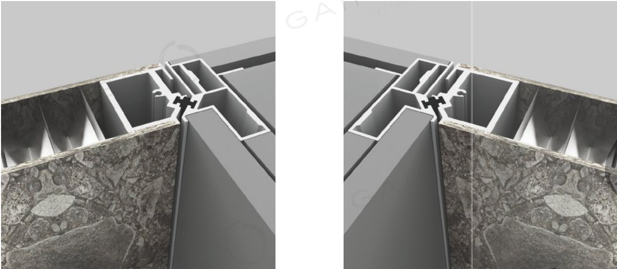
STM019型材图
