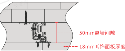
墙板离墙最少值50mm
