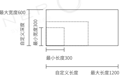
MK029尺寸范围
