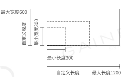
MK070尺寸范围
