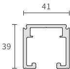
移门吊轨
